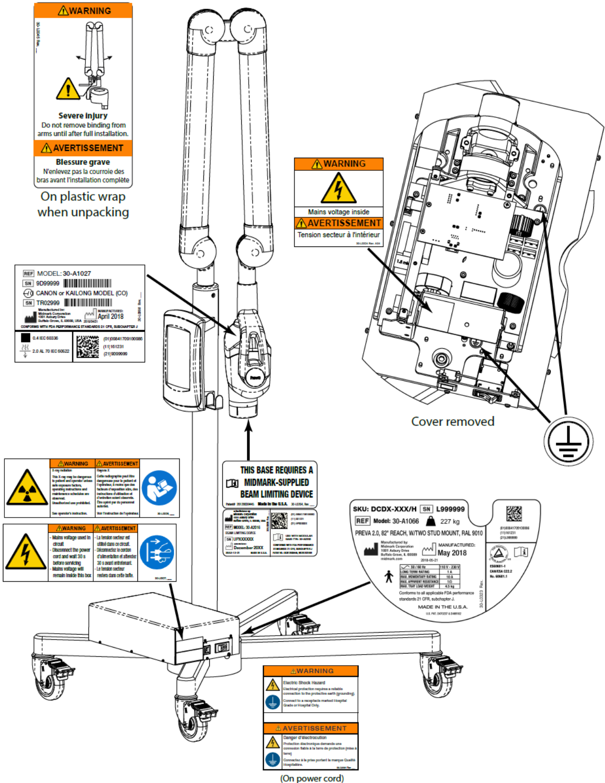
Overview of Mobile Configuration DC Generator Labels
