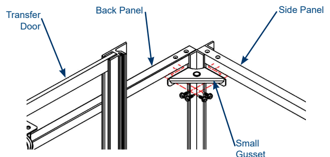
BACK/SIDE PANEL CONNECTION
