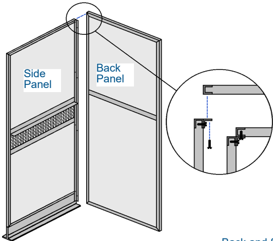
Back and Side Panel Connection
