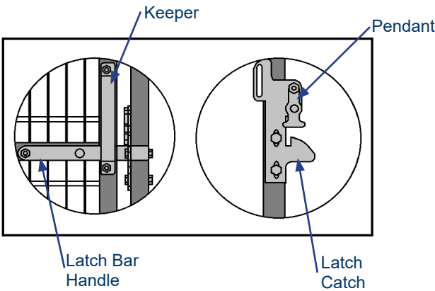
SS GATE/SIDELIGHT LATCH
