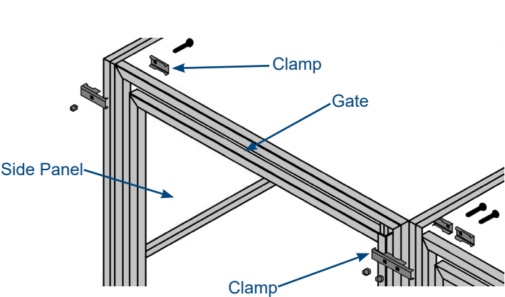
GATE PANEL ASSEMBLY
