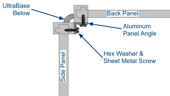
BACK AND SIDE PANEL ASSEMBLY
