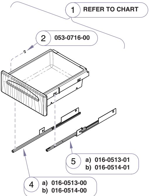
Integrated Handle
