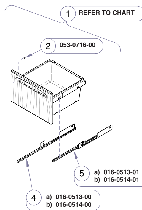
Integrated Handle
